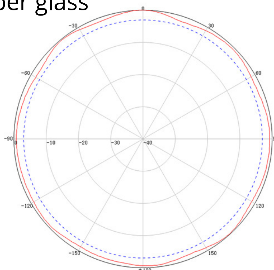
Horizontal Pattern
